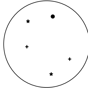
Kusken
