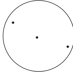
Andromeda
